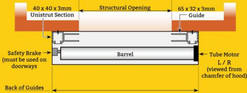
Top view of face fix shutter
