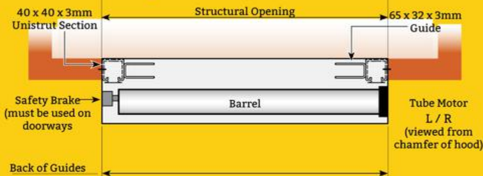
Top view of reveal fix shutter
